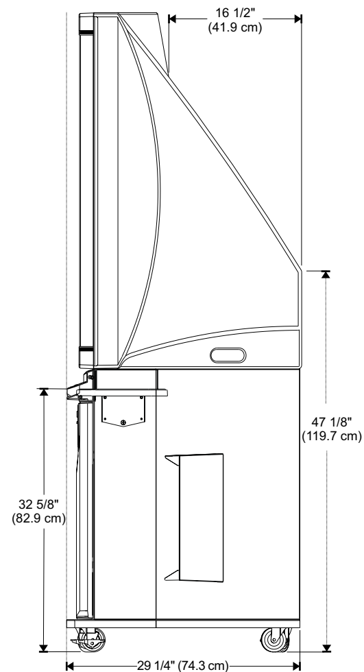
Side View
